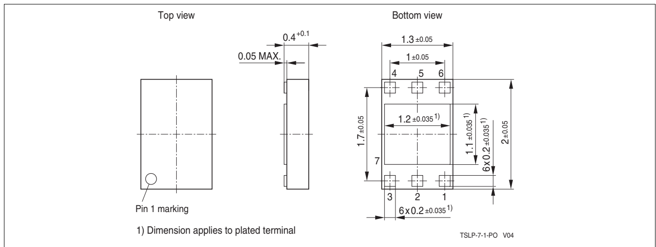
Figure 8-1 Package Outline
