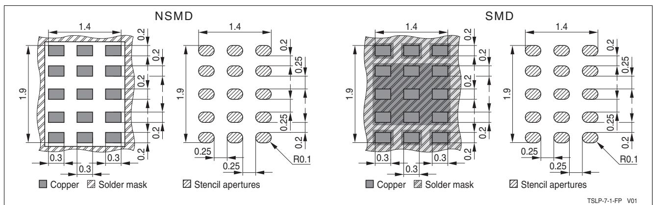
Figure 8-2 Package Footprint
