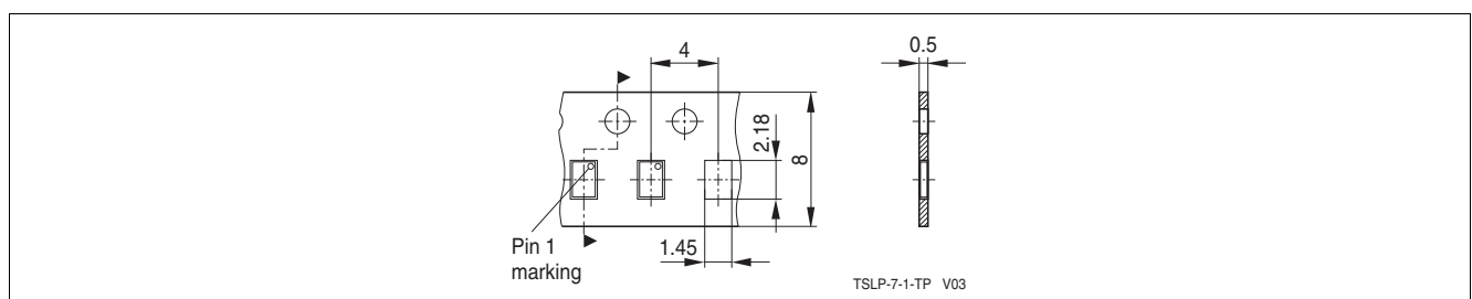
Figure 8-4 Tape Dimensions
